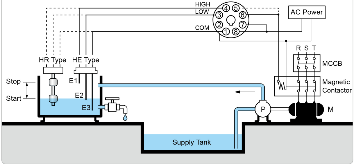
HLC-200A Connection Diagram
