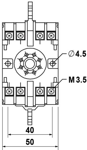
< HLC-200A Socket >
