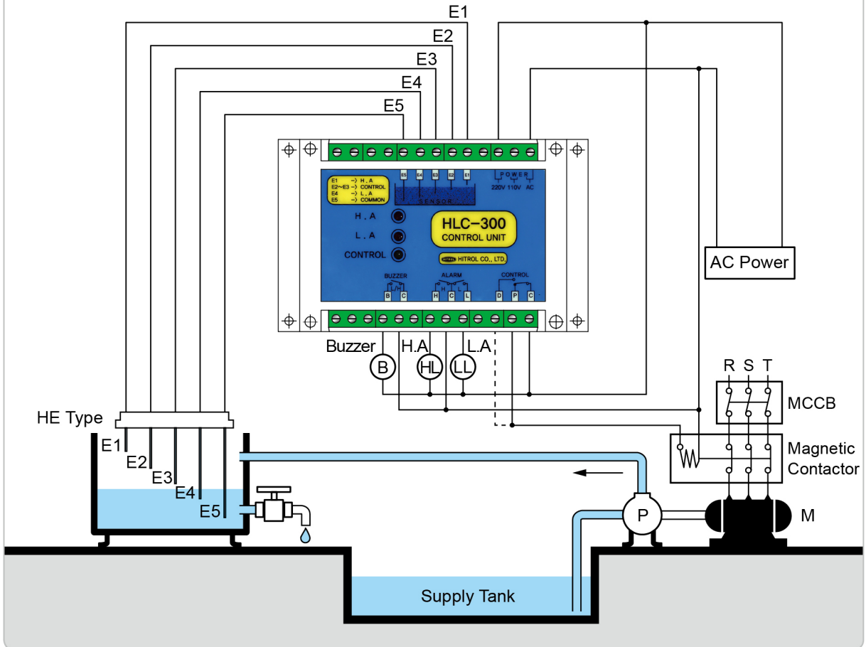
HLC-300 Connection Diagram
